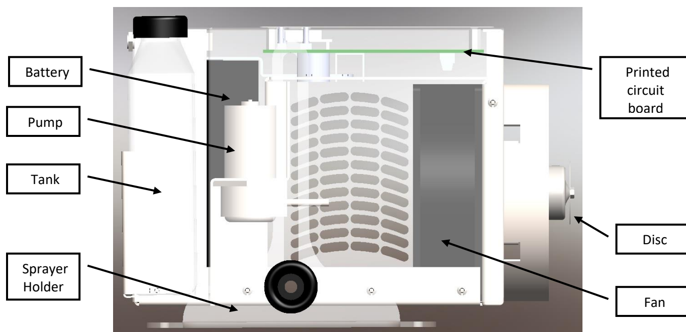
Figure 1: diffuser components
