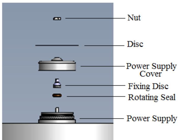
Figure 6 : Disc replacement
